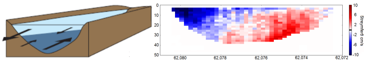
Figure 2 Left) Typical flow pattern in Faroese fjords dominated by estuarine circulation influenced by the coriolis force; from (Hansen, 2000). Right) Flow in Sørvágsfjørður measured in a calm weather situation demonstrates estuarine flow. Red is inflow, blue is outflow; from (á Norði and Patursson, 2017).
