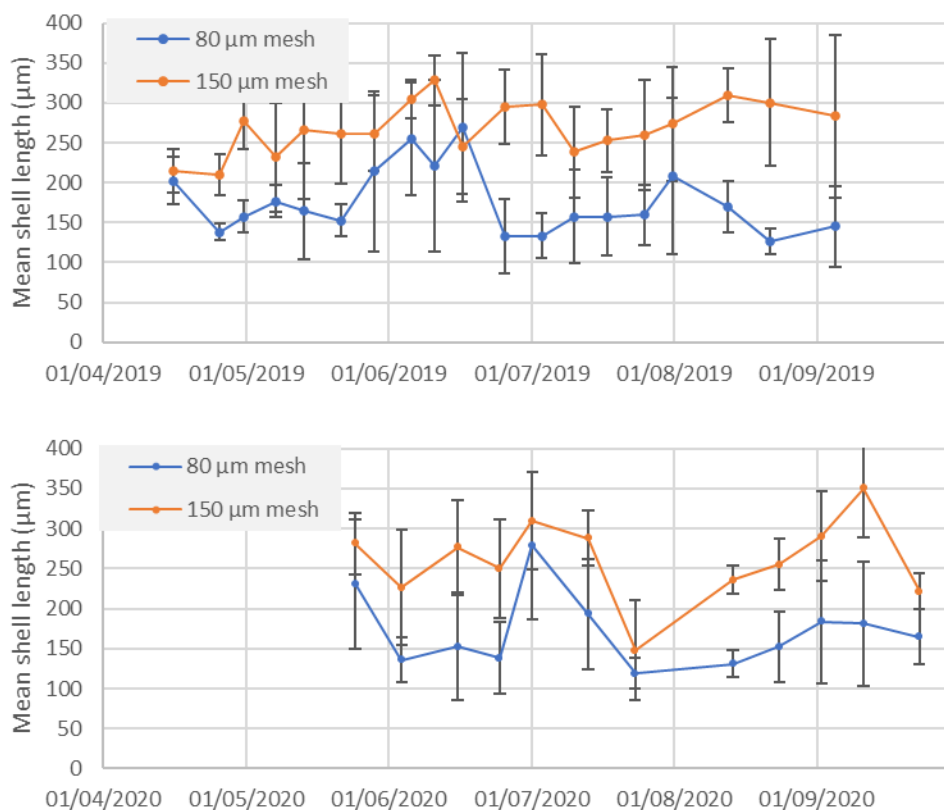
Figure 4 Mean shell length at station SO 6 from vertical hauls from 8 m depth to the surface with the 80 \mu\text{m} and 150 \mu\text{m} plankton net. Samples from 2019 are shown in the upper figure while the lower figure shows the samples from 2020. Error bars show the standard deviation.
